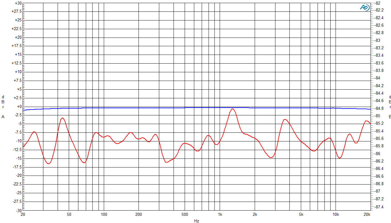
Figure 17: Crosstalk
