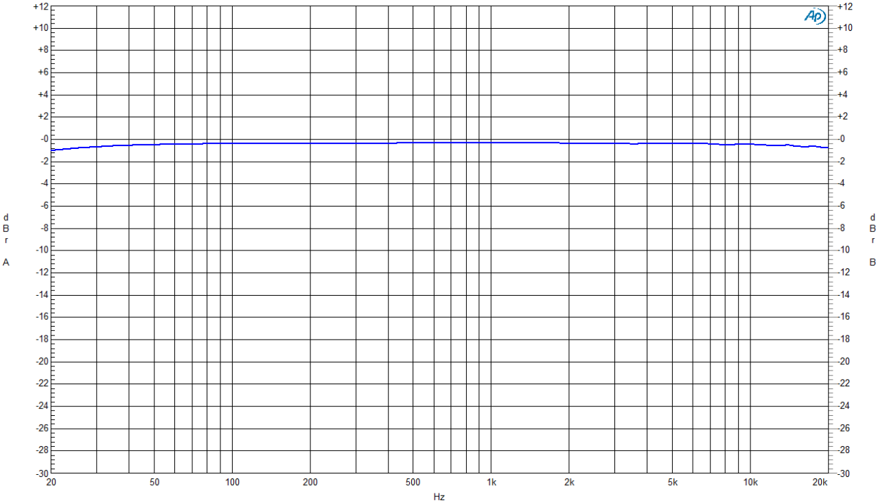
Figure 14: Frequency Response
