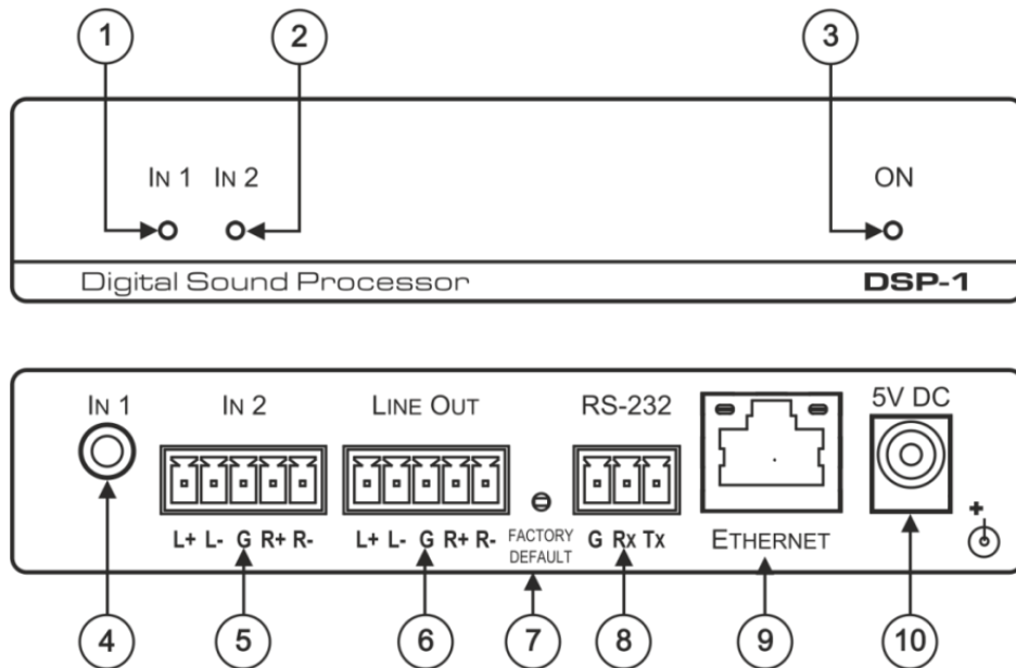
Figure 1: DSP-1 Digital Sound Processor
