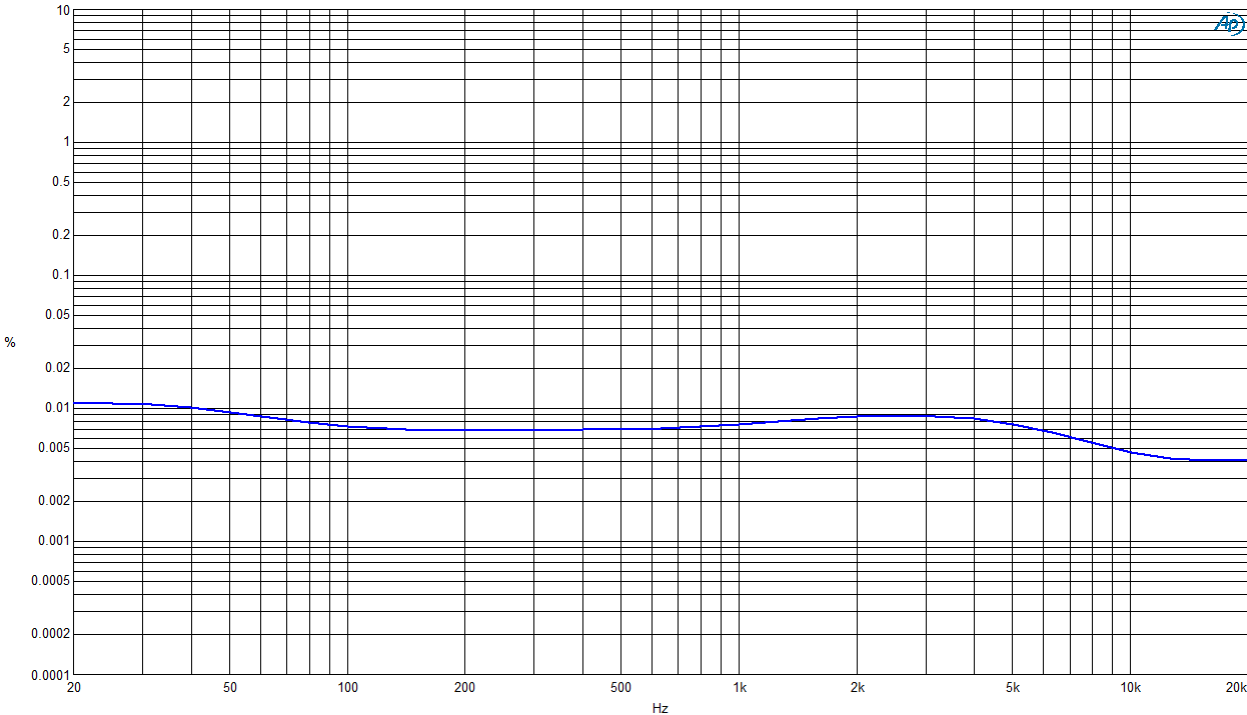
Figure 16: THD + N
